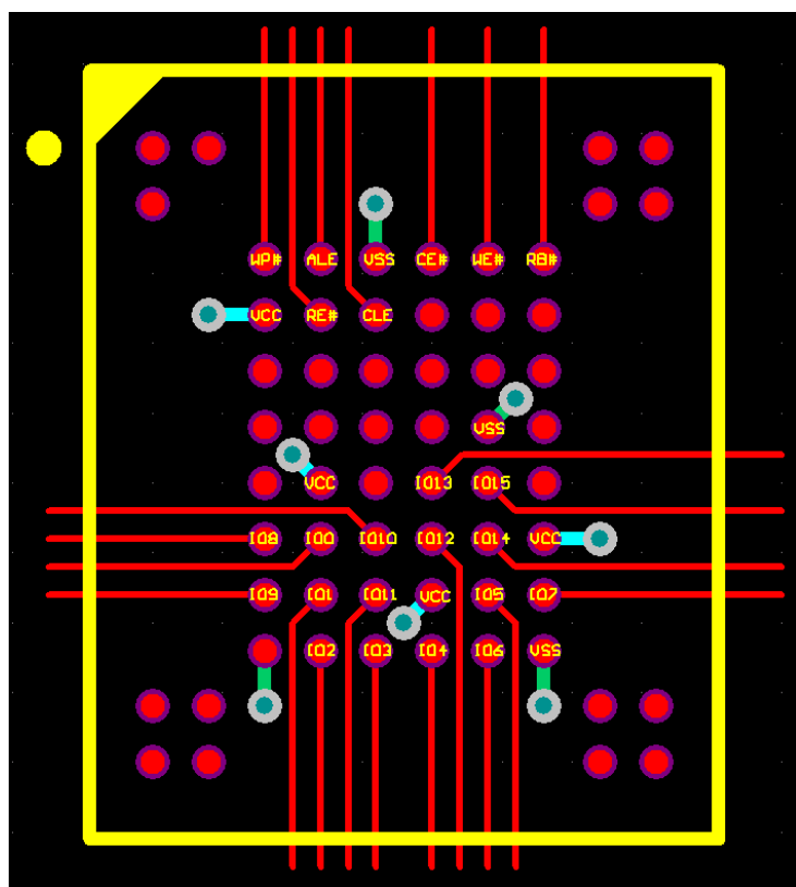
Figure 1 FBGA 63 PCB breakout (Top View, Balls Down)
