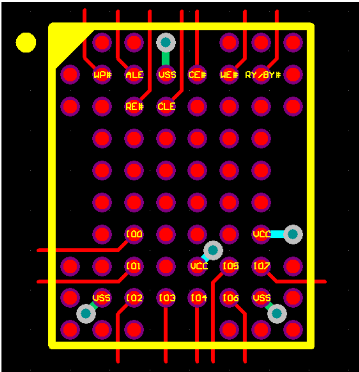
Figure 2 FBGA 67 PCB breakout (Top view, balls down)
