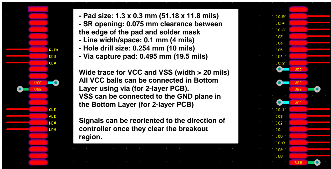
Figure 3 TSOP Land pattern (x8, x16)
